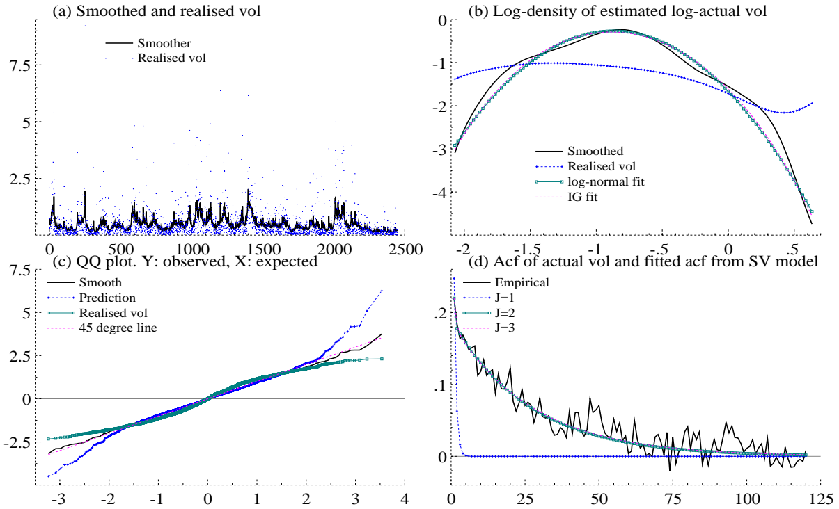
Figure 4: Results from the fit of the SV model using M=6 (4 hour returns) on the 5 minute Olsen data. (a) gives the time series of realised volatilities \{y\}_n together with the smoothed estimates of actual volatility. (b) draws the kernel based estimates of the log-density of log-realised volatility and log-smoothed log-actual volatility. Also drawn are the log-normal and inverse Gaussian fits. These lines are so close they appear to be almost on top of one another. (c) QQ plot for returns divided by estimated actual vol, using realised, predicted and smoothed volatility. Perfect fit sits on a 45^\circ line. (d) Acf of realised volatility and the fit of SV model with various superpositions of J processes. Code is available at ssf_empirical.ox .
