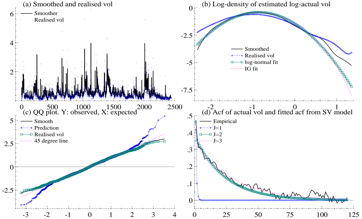
Figure 5: Results from the fit of the SV model using M=144 (10 minute returns) on the 5 minute Olsen data. (a) gives \{y\}_n together with the smoothed estimates of actual volatility. (b) draws the estimates of the log-density of log-realised volatility and log-smoothed log-actual volatility. Also log-normal and inverse Gaussian fits. (c) QQ plot for standardised returns. (d) Acf of realised volatility and the fit of SV model with various superpositions of J processes. Code is available at ssf_empirical.ox .
