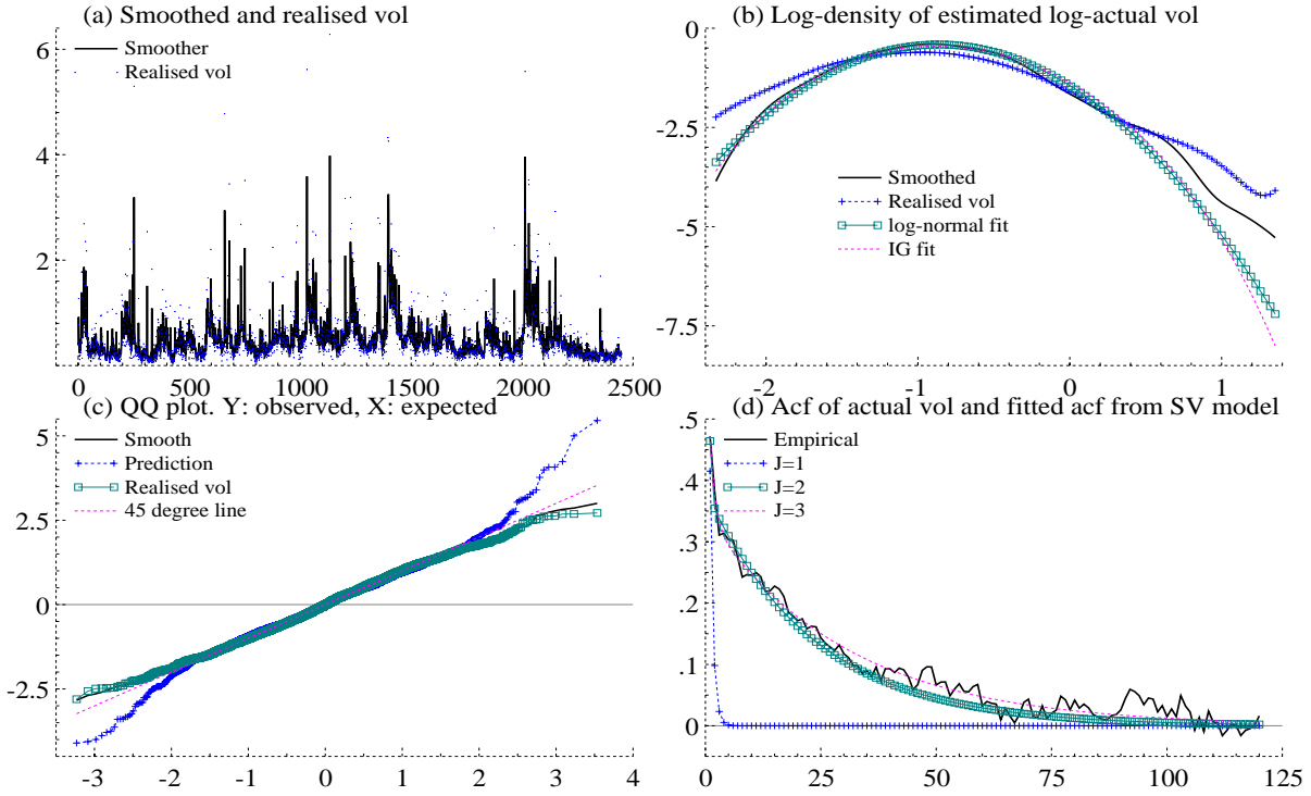
Figure 6: Results from the fit of the SV model using M=18 (80 minute returns) on the 5 minute Olsen data. (a) gives \{y\}_n together with the smoothed estimates of actual volatility. (b) draws the estimates of the log-density of log-realised volatility and log-smoothed log-actual volatility. Also log-normal and inverse Gaussian fits. (c) QQ plot for standardised returns. (d) Acf of realised volatility and the fit of SV model with various superpositions of J processes. Code is available at ssf_empirical.ox .
