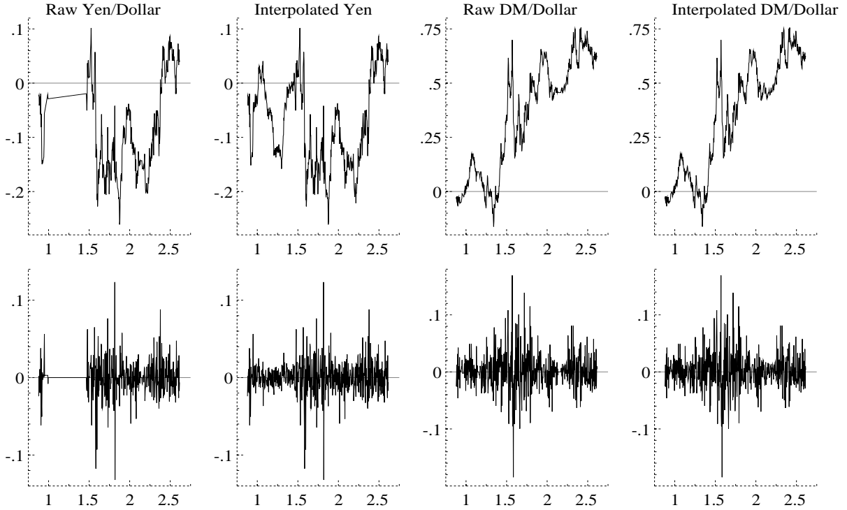
Figure 7: Top line of graphs are the raw and interpolated data using a Brownian bridge interpolator. Bottom line of graphs is the corresponding returns. The x-axes are marked off in days.
